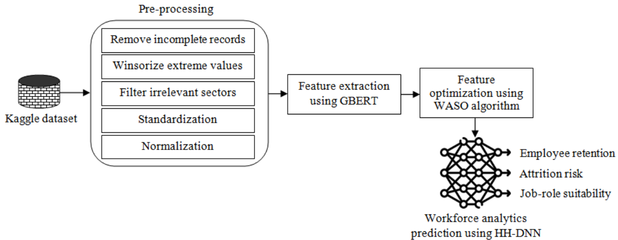
Figure 1. Security-aware analytics model (GBERT–WASO–HH-DNN) for workforce management
