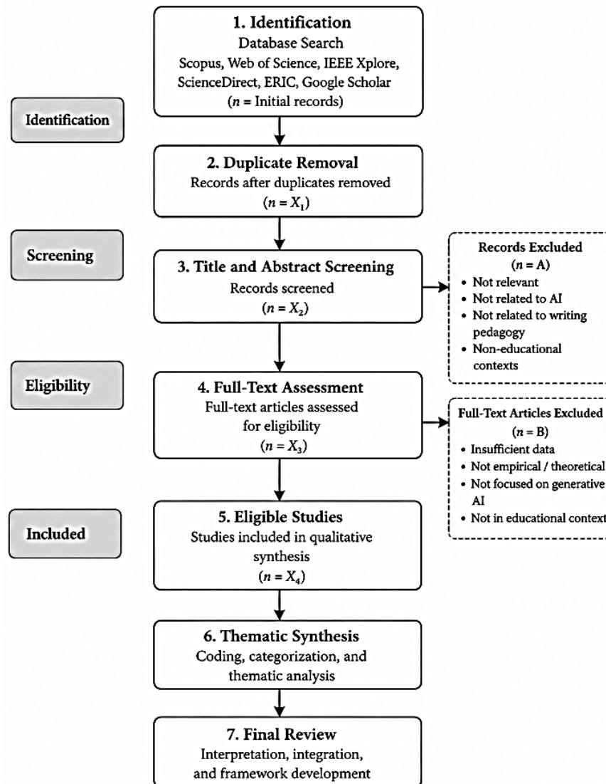
Figure 1. Methodology of Structured literature review (PRISMA-informed)
